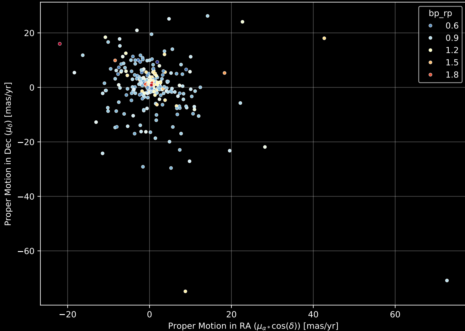
GALAH DR4 Field: [2858] Proper Motion Diagram (n= 267)
