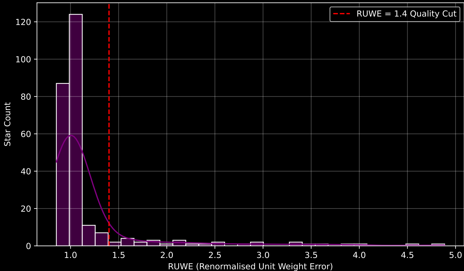
GALAH DR4 Field [2858] RUWE Distribution (n= 259)
