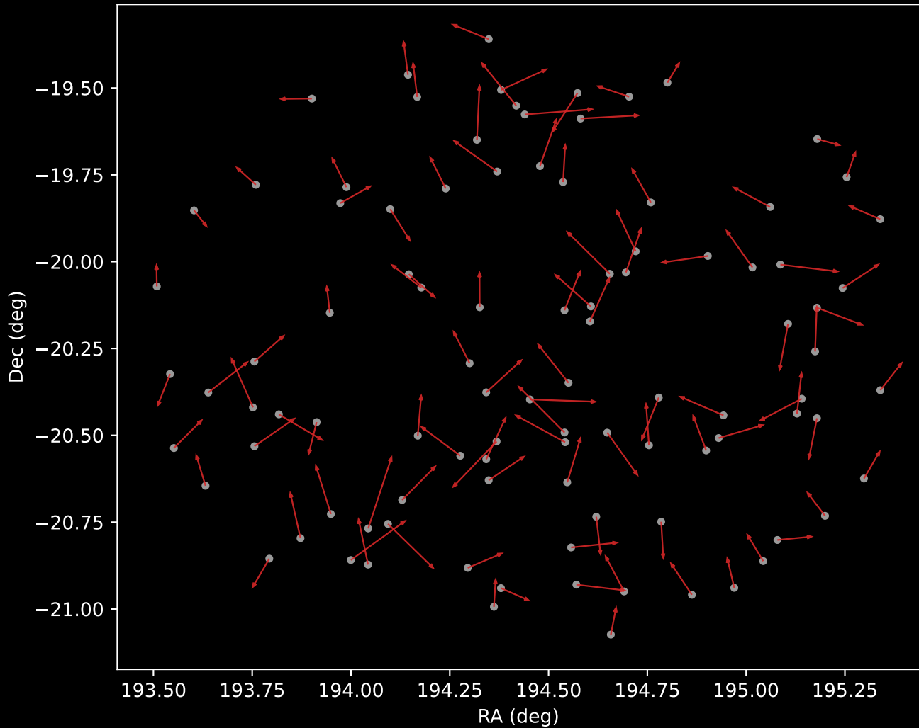
GALAH DR4 Cluster 6 Proper Motion Vectors (n=98)
