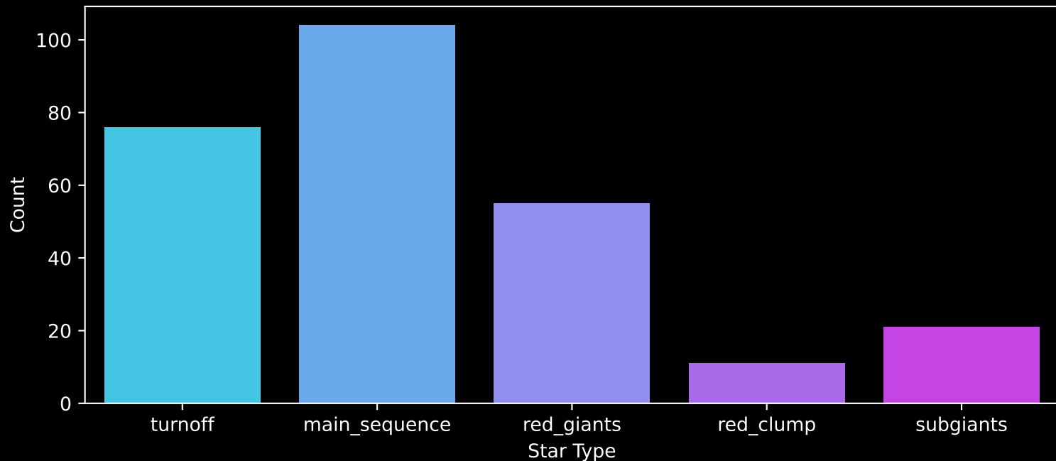
GALAH DR4 Field: [2858] Count plot of Star Type
